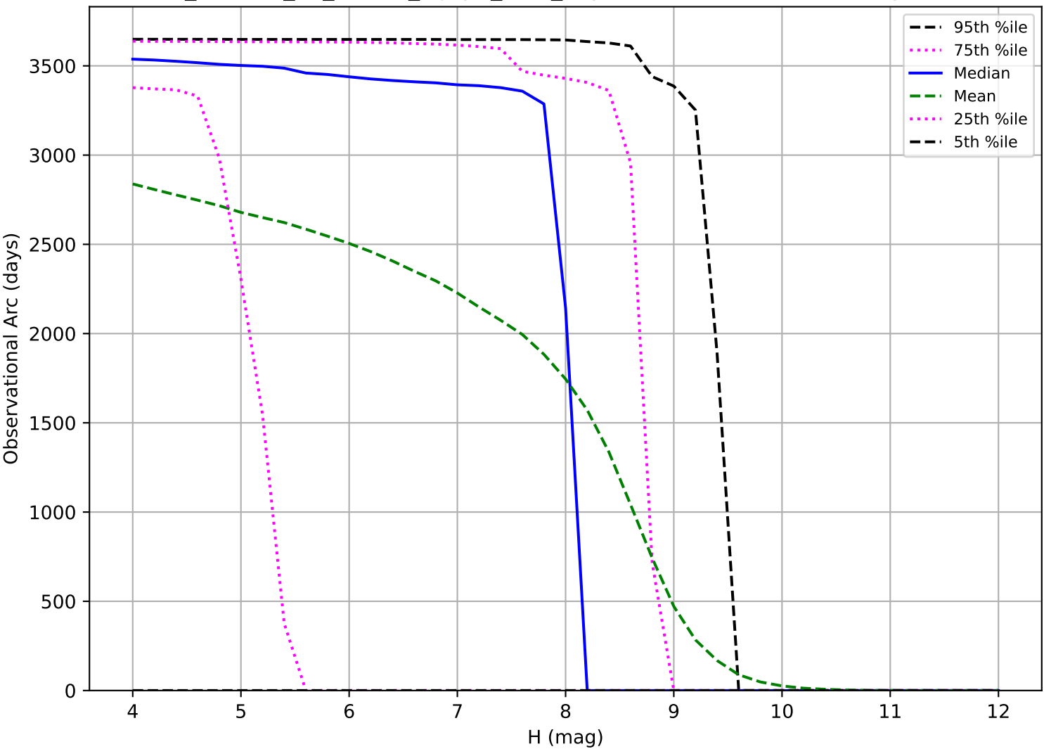
roll_uniform_eh_acc0.0_mjdp0_v3.4_10yrs: Observational Arc Length TNO
