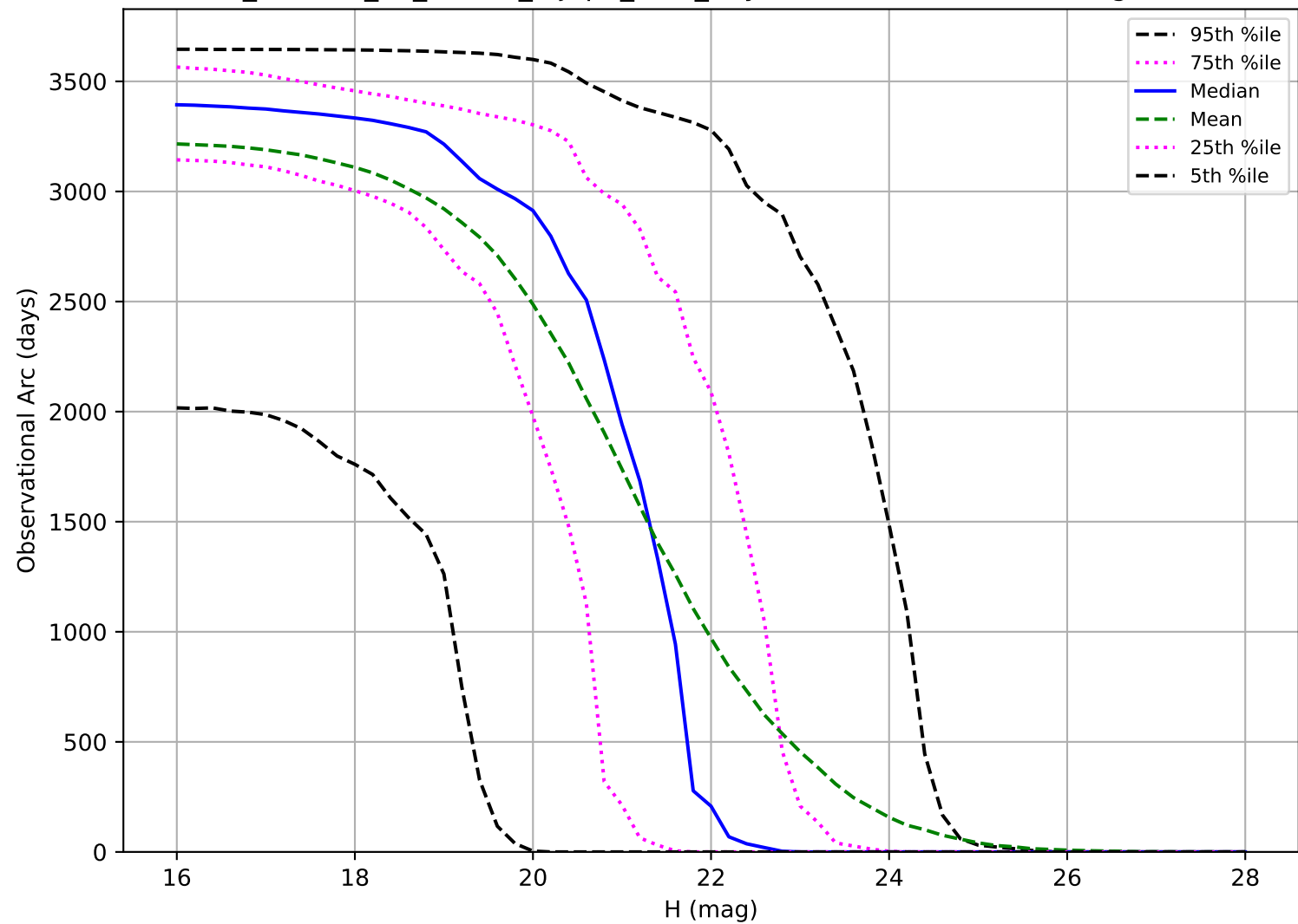
roll_uniform_eh_acc0.0_mjdp0_v3.4_10yrs: Observational Arc Length PHA
