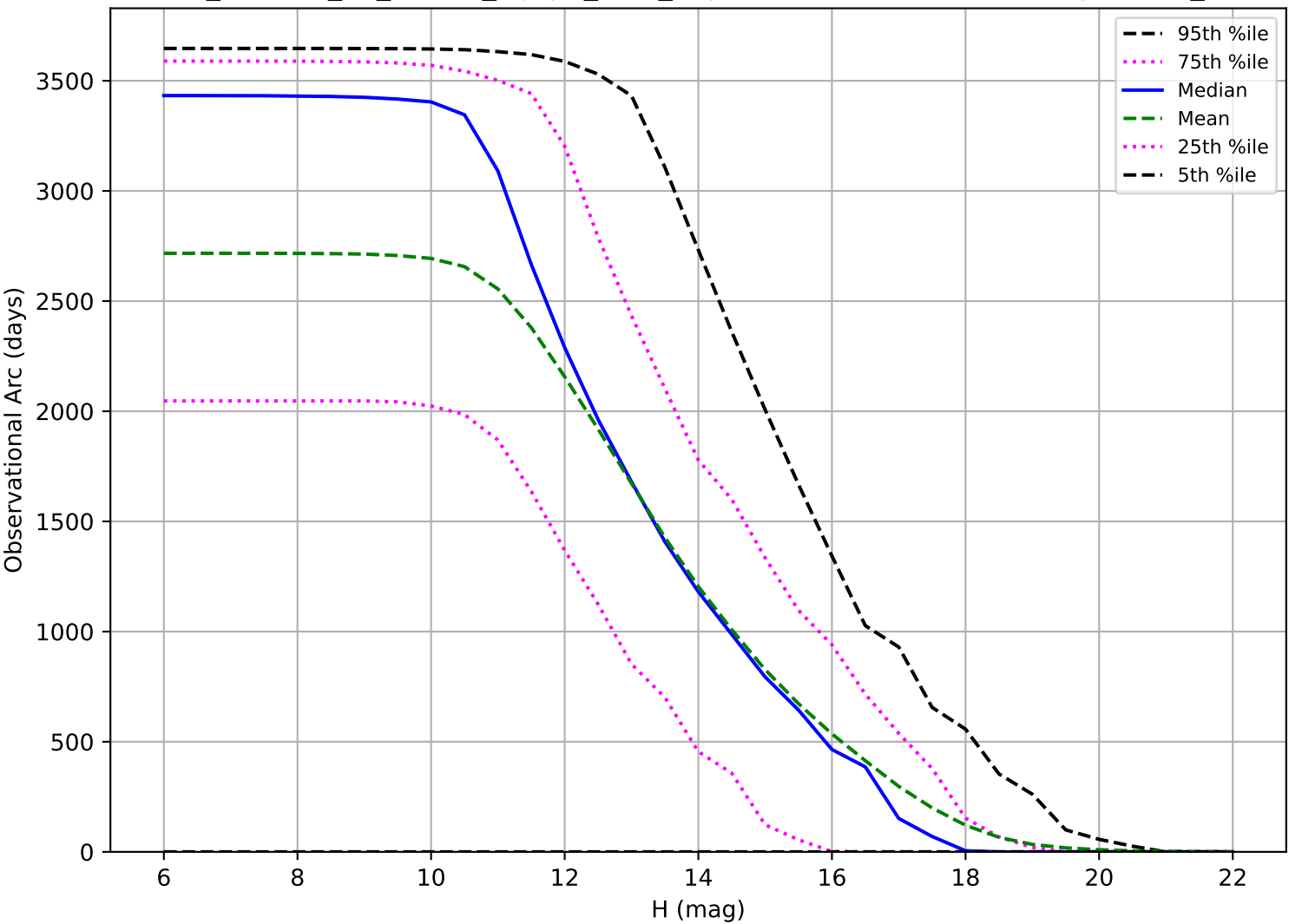
roll_uniform_eh_acc0.0_mjdp0_v3.4_10yrs: Observational Arc Length OCC_r5
