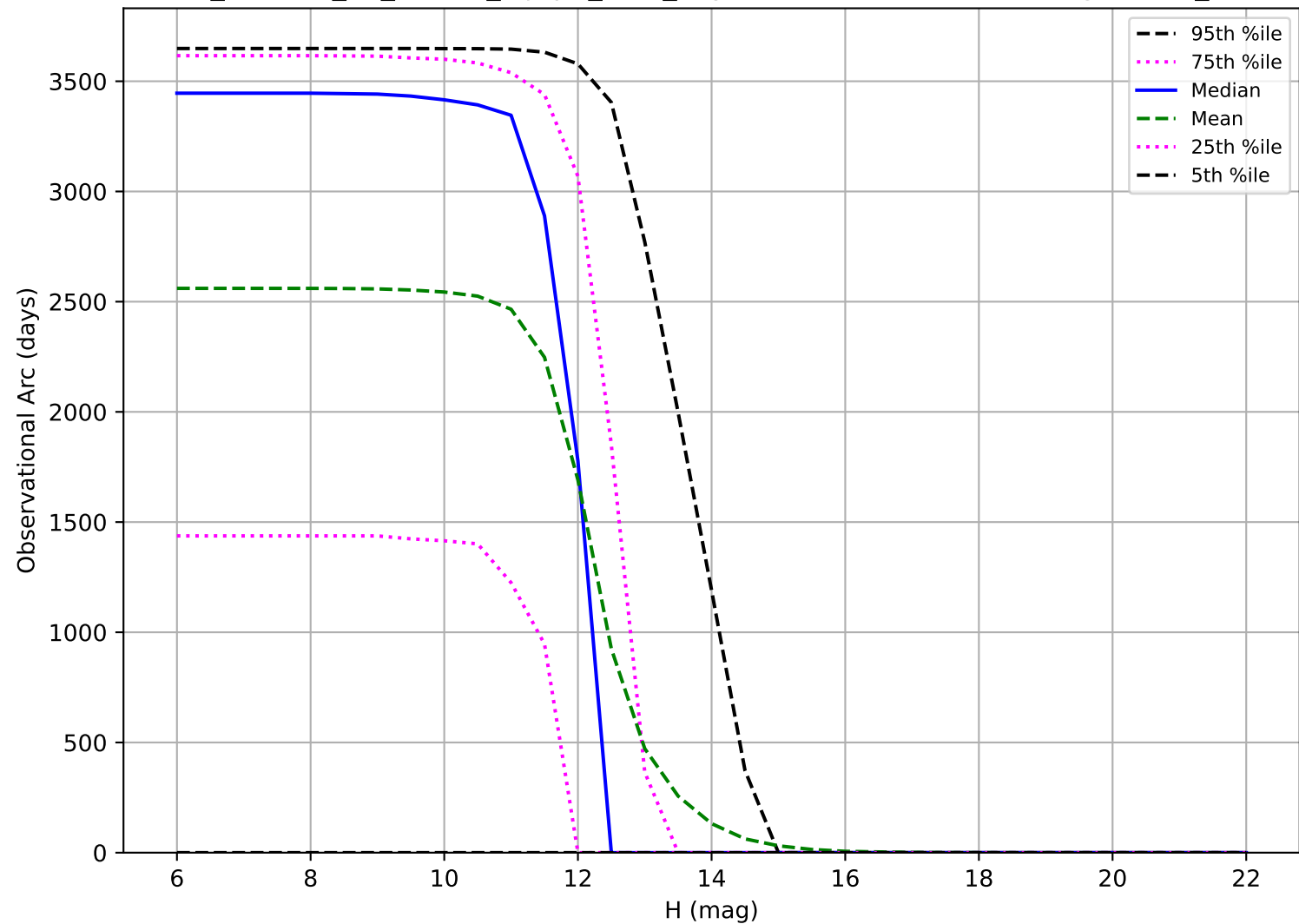
roll_uniform_eh_acc0.0_mjdp0_v3.4_10yrs: Observational Arc Length OCC_r20
