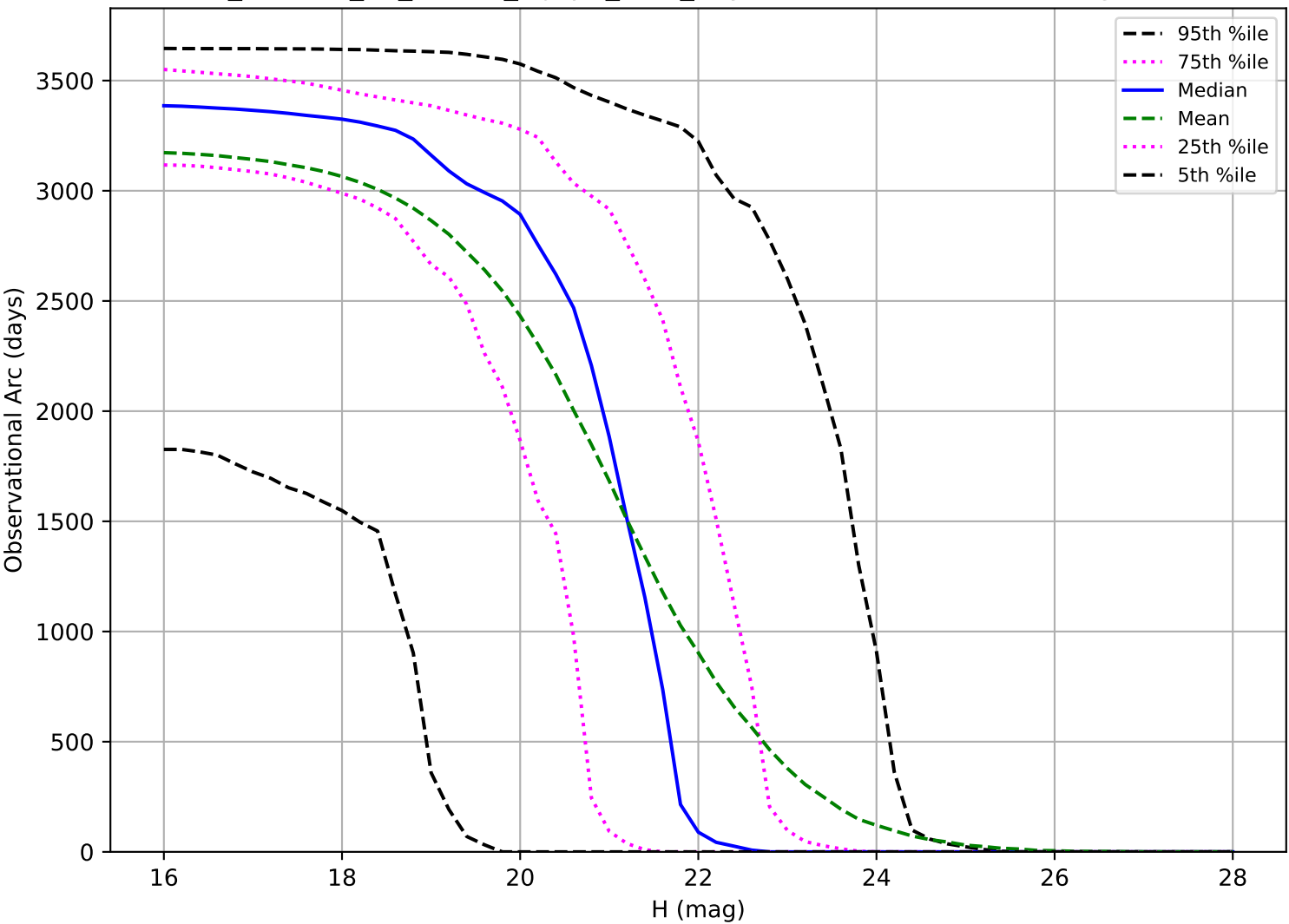
roll_uniform_eh_acc0.0_mjdp0_v3.4_10yrs: Observational Arc Length NEO
