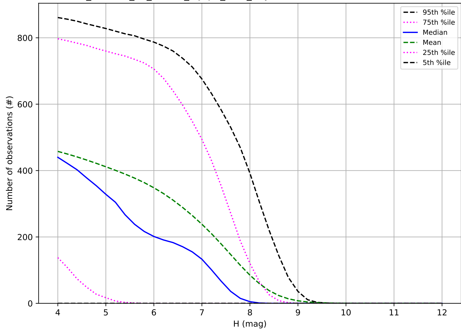
roll_uniform_eh_acc0.0_mjdp0_v3.4_10yrs: Number of observations TNO
