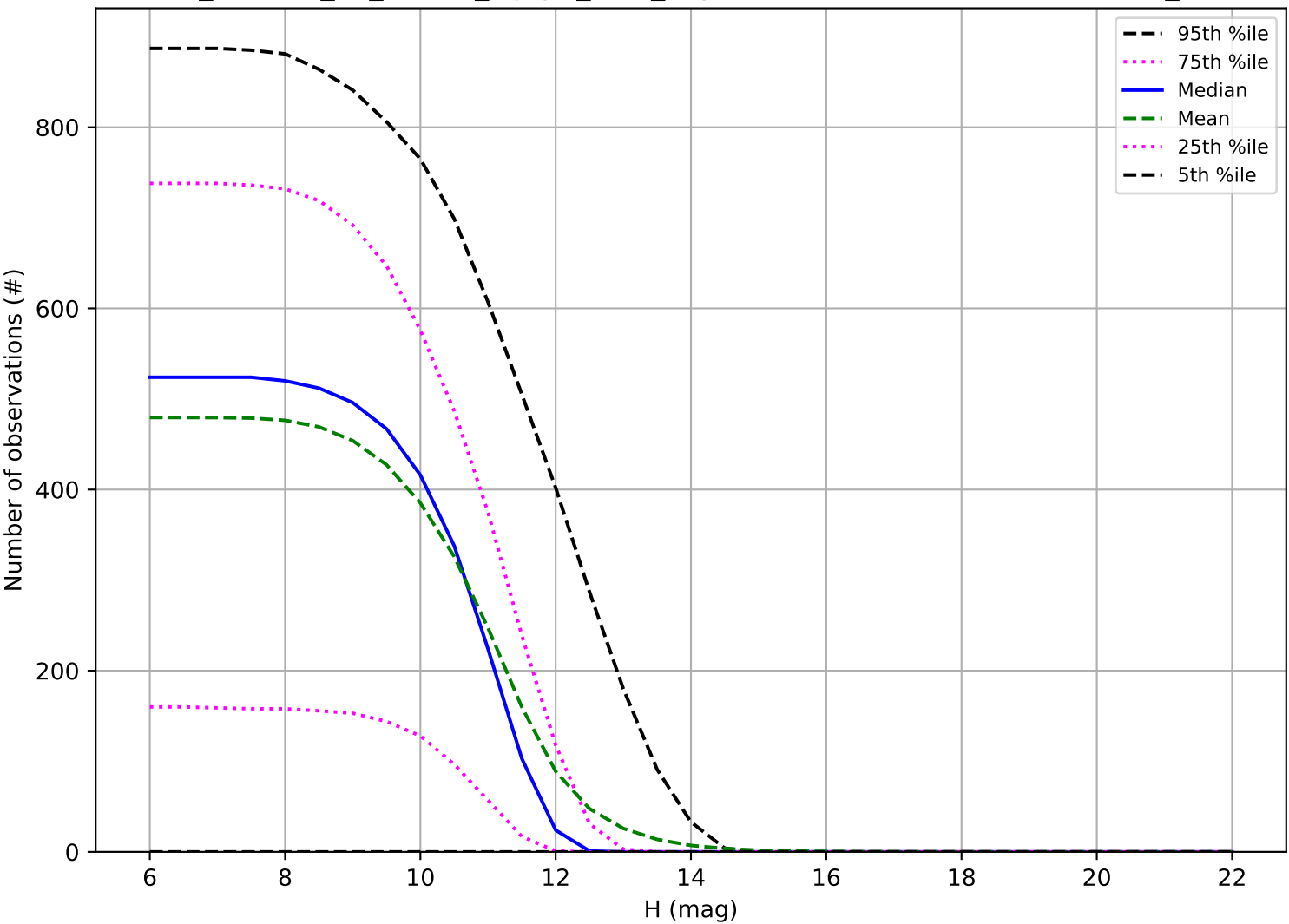
roll_uniform_eh_acc0.0_mjdp0_v3.4_10yrs: Number of observations OCC_r20
