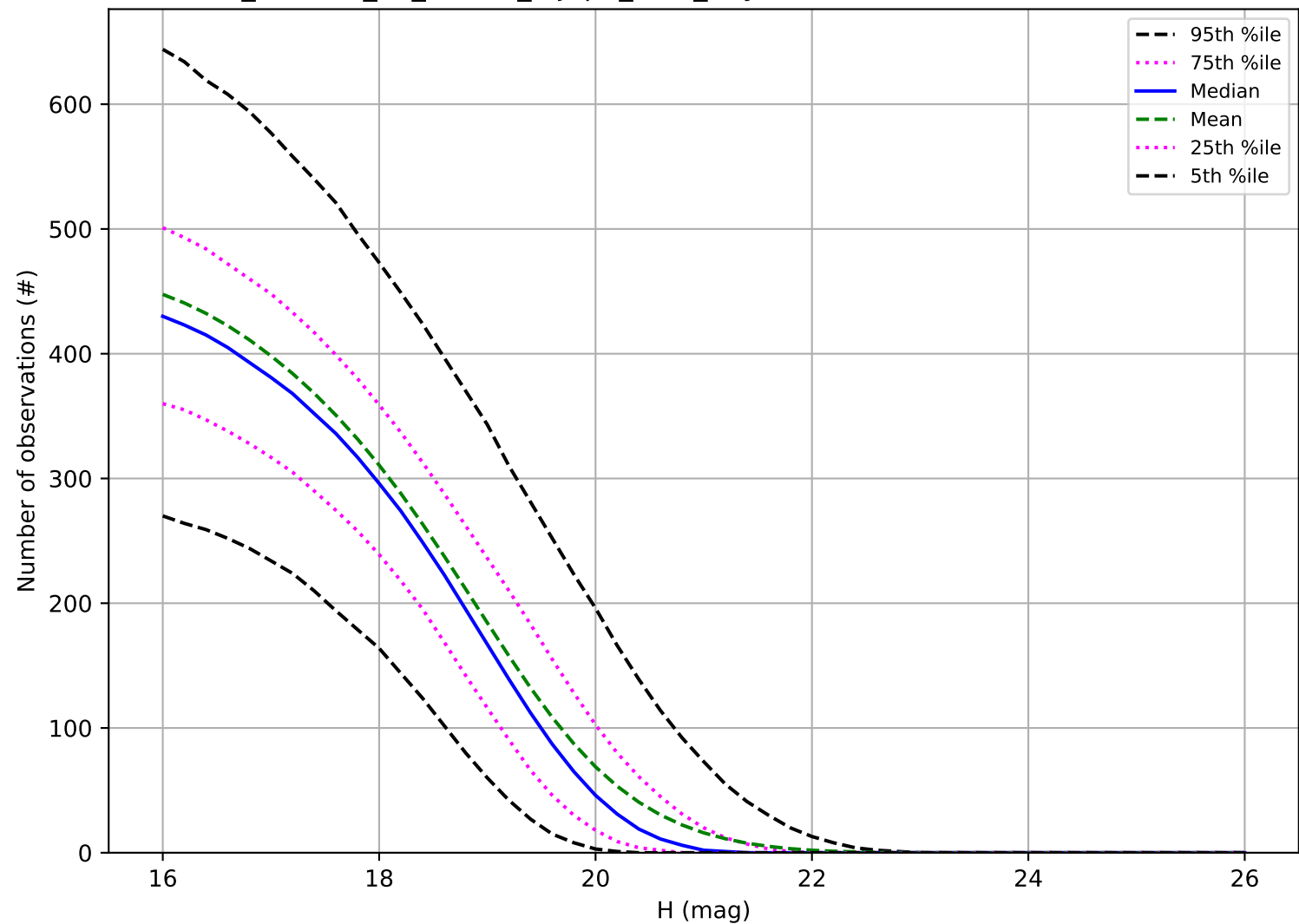
roll_uniform_eh_acc0.0_mjdp0_v3.4_10yrs: Number of observations MBA
