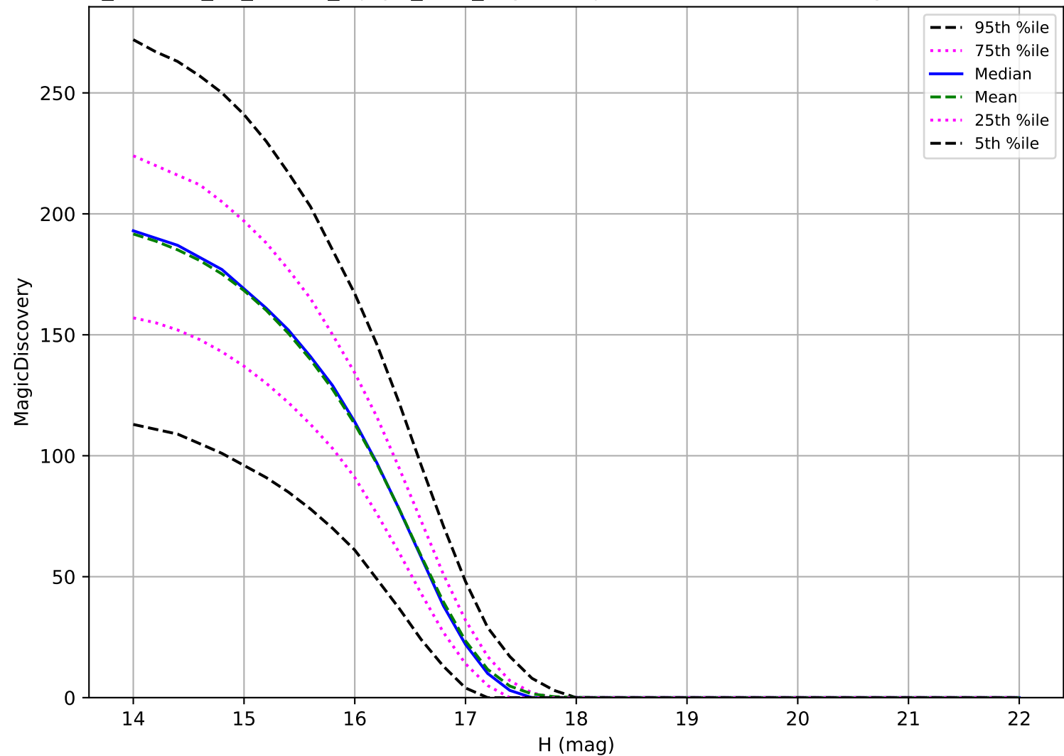
roll_uniform_eh_acc0.0_mjdp0_v3.4_10yrs: Trojan 6 detections in 60 nights detection loss
