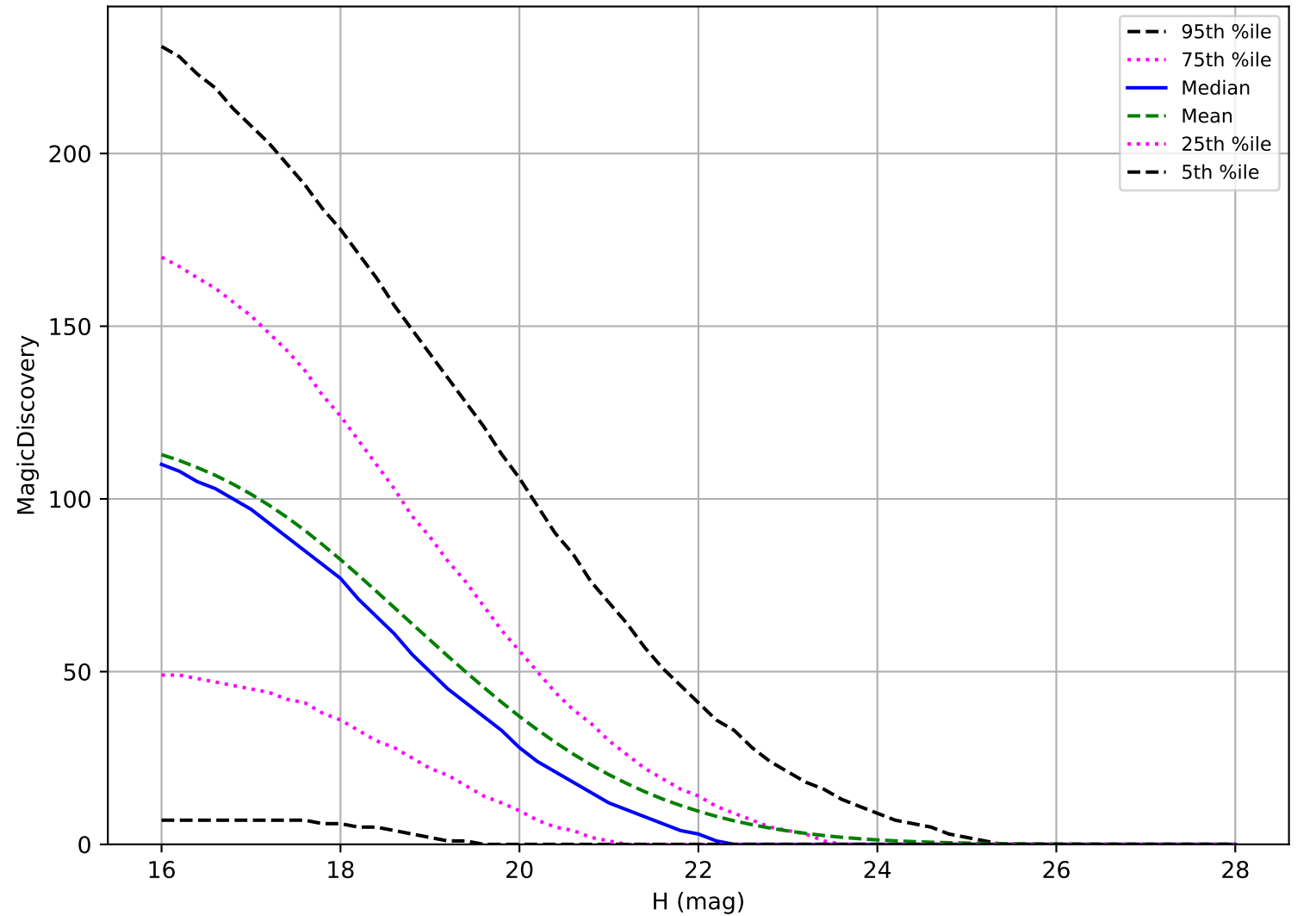
roll_uniform_eh_acc0.0_mjdp0_v3.4_10yrs: PHA 6 detections in 60 nights detection loss
