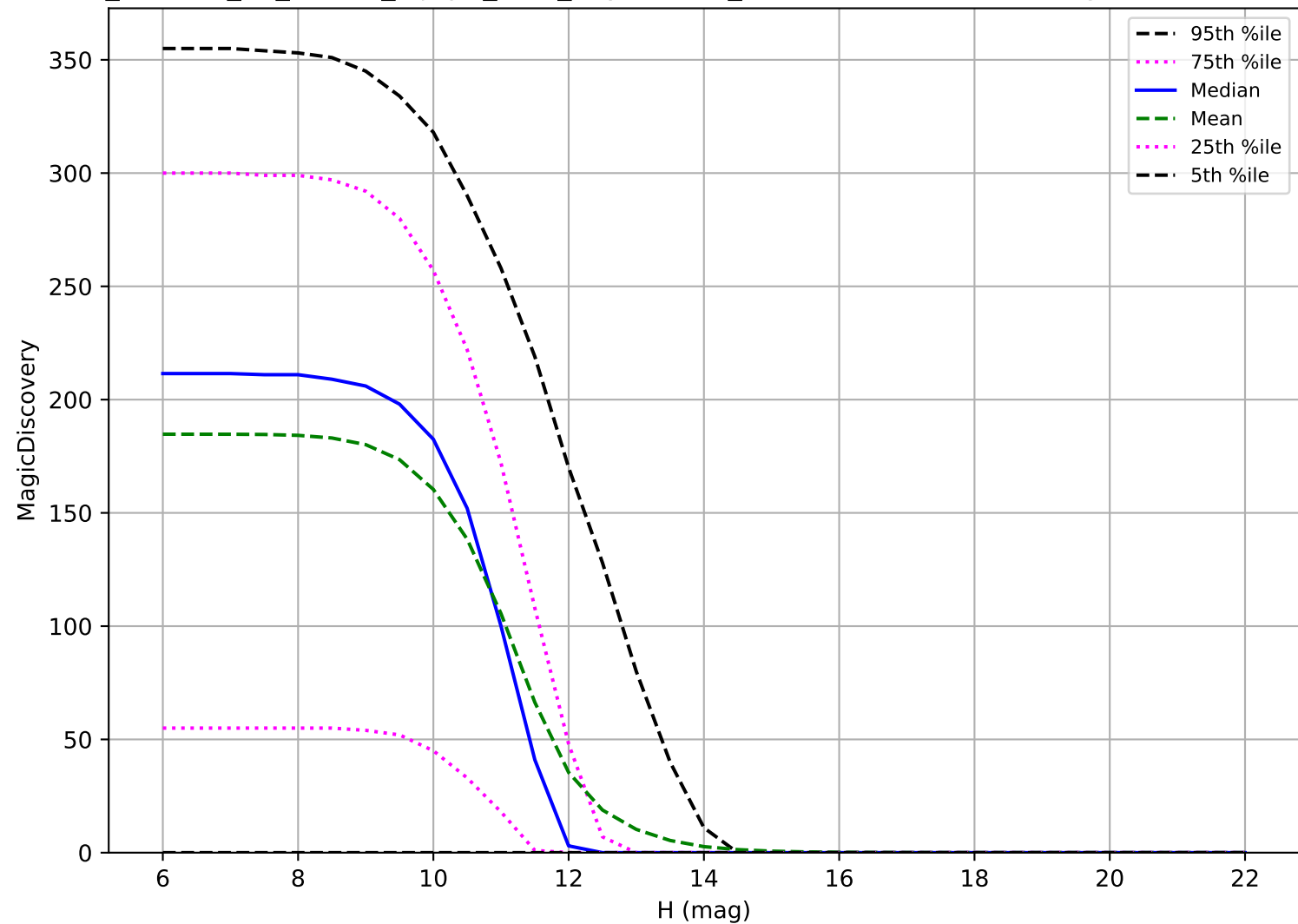
roll_uniform_eh_acc0.0_mjdp0_v3.4_10yrs: OCC_r20 6 detections in 60 nights detection loss
