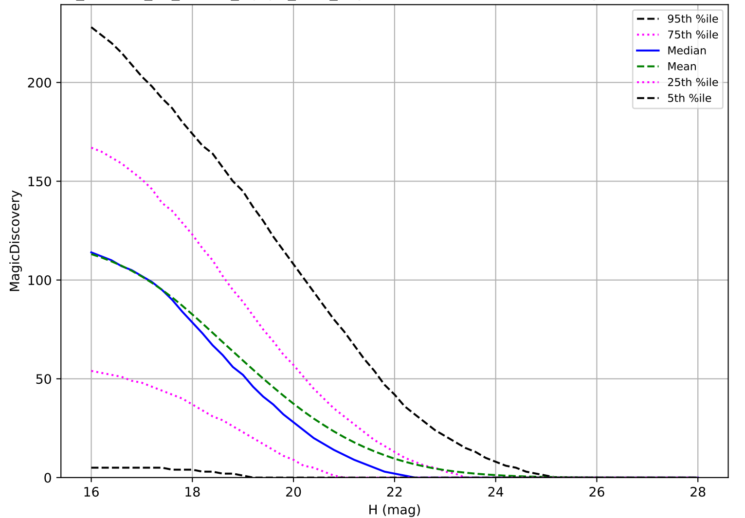
roll_uniform_eh_acc0.0_mjdp0_v3.4_10yrs: NEO 6 detections in 60 nights detection loss
