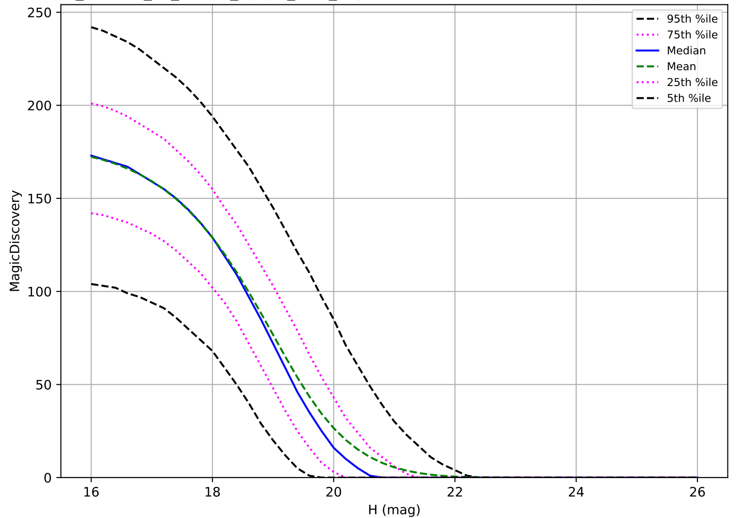
roll_uniform_eh_acc0.0_mjdp0_v3.4_10yrs: MBA 6 detections in 60 nights detection loss
