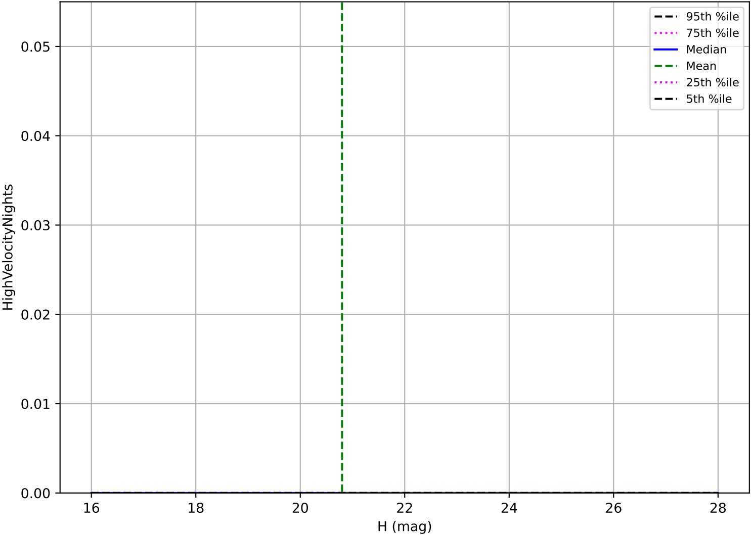
roll_uniform_eh_acc0.0_mjdp0_v3.4_10yrs: Vatira High velocity pair detection loss
