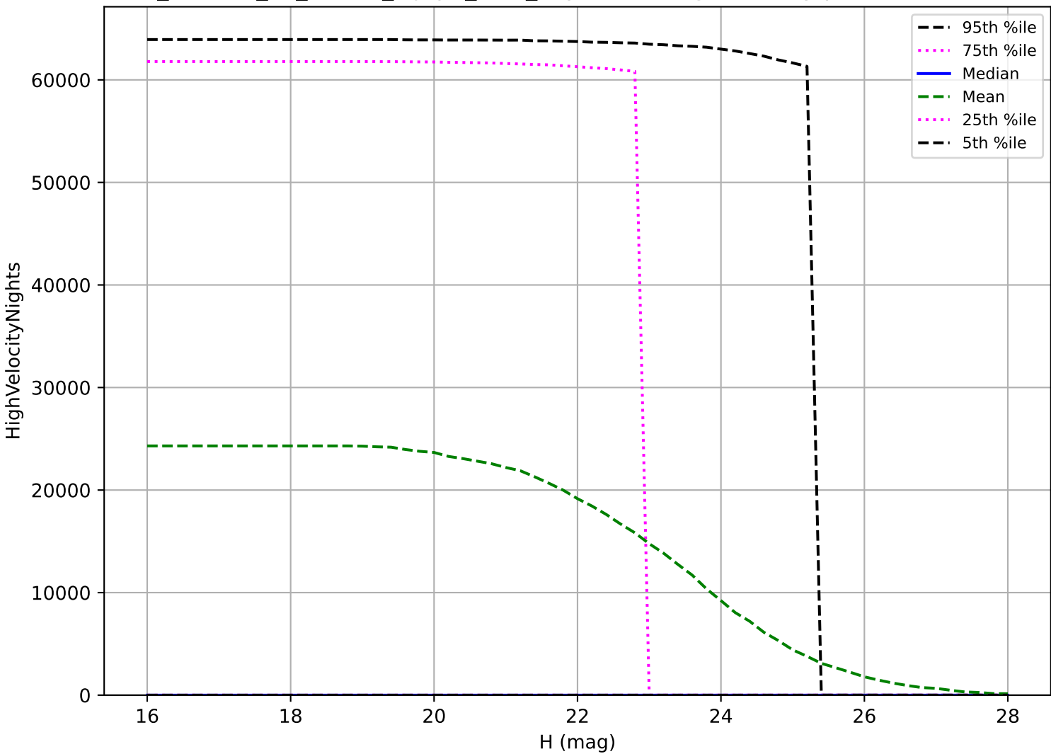
roll_uniform_eh_acc0.0_mjdp0_v3.4_10yrs: PHA High velocity pair detection loss
