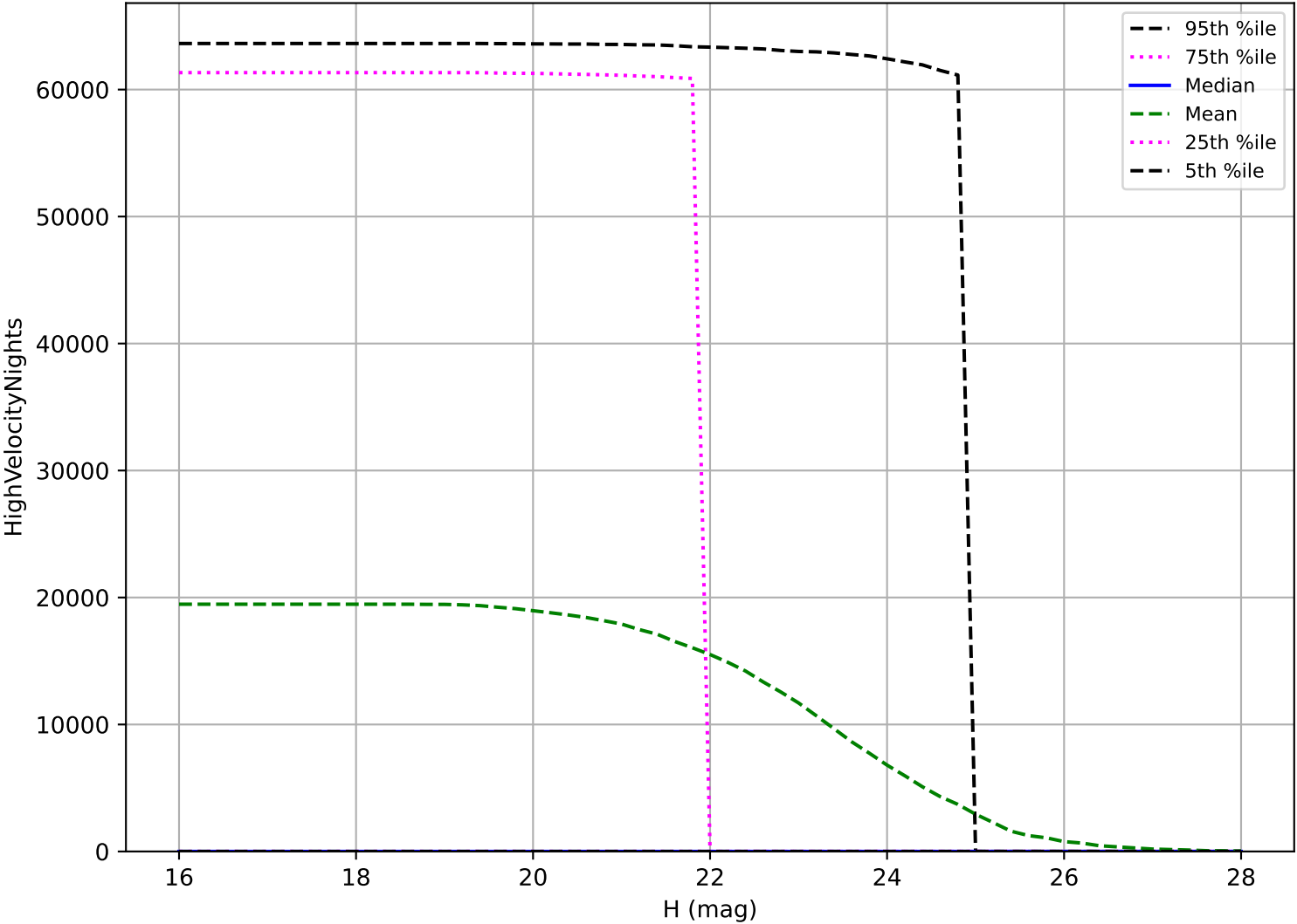
roll_uniform_eh_acc0.0_mjdp0_v3.4_10yrs: NEO High velocity pair detection loss
