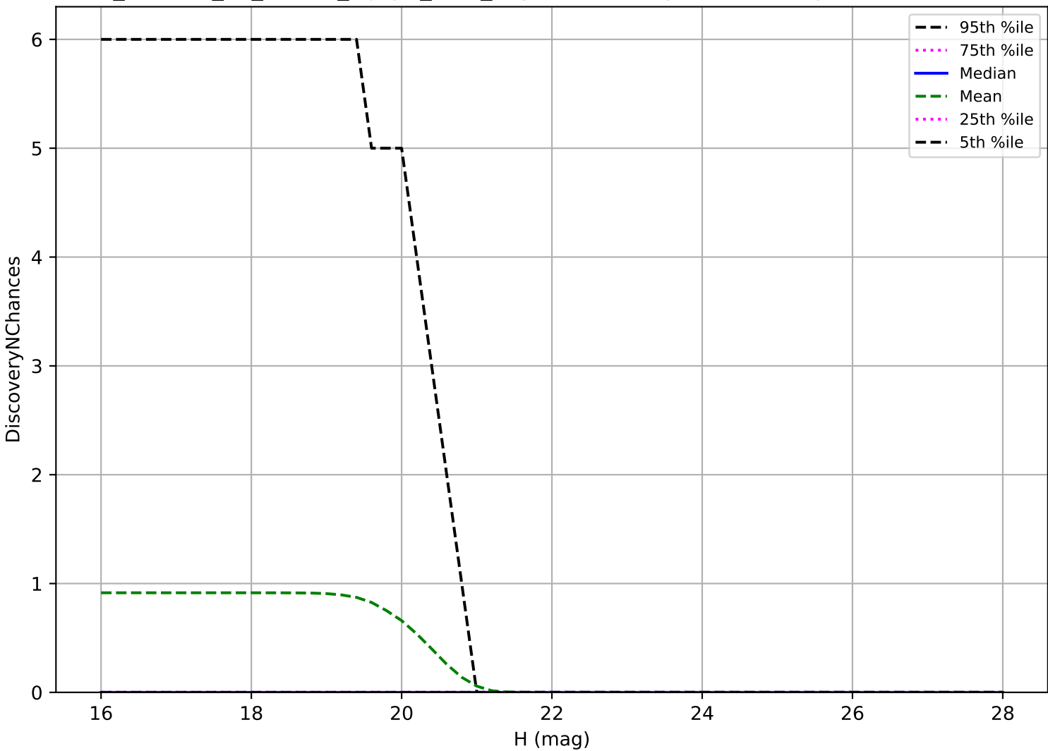
roll_uniform_eh_acc0.0_mjdp0_v3.4_10yrs: Vatira 3 pairs in 15 nights detection loss
