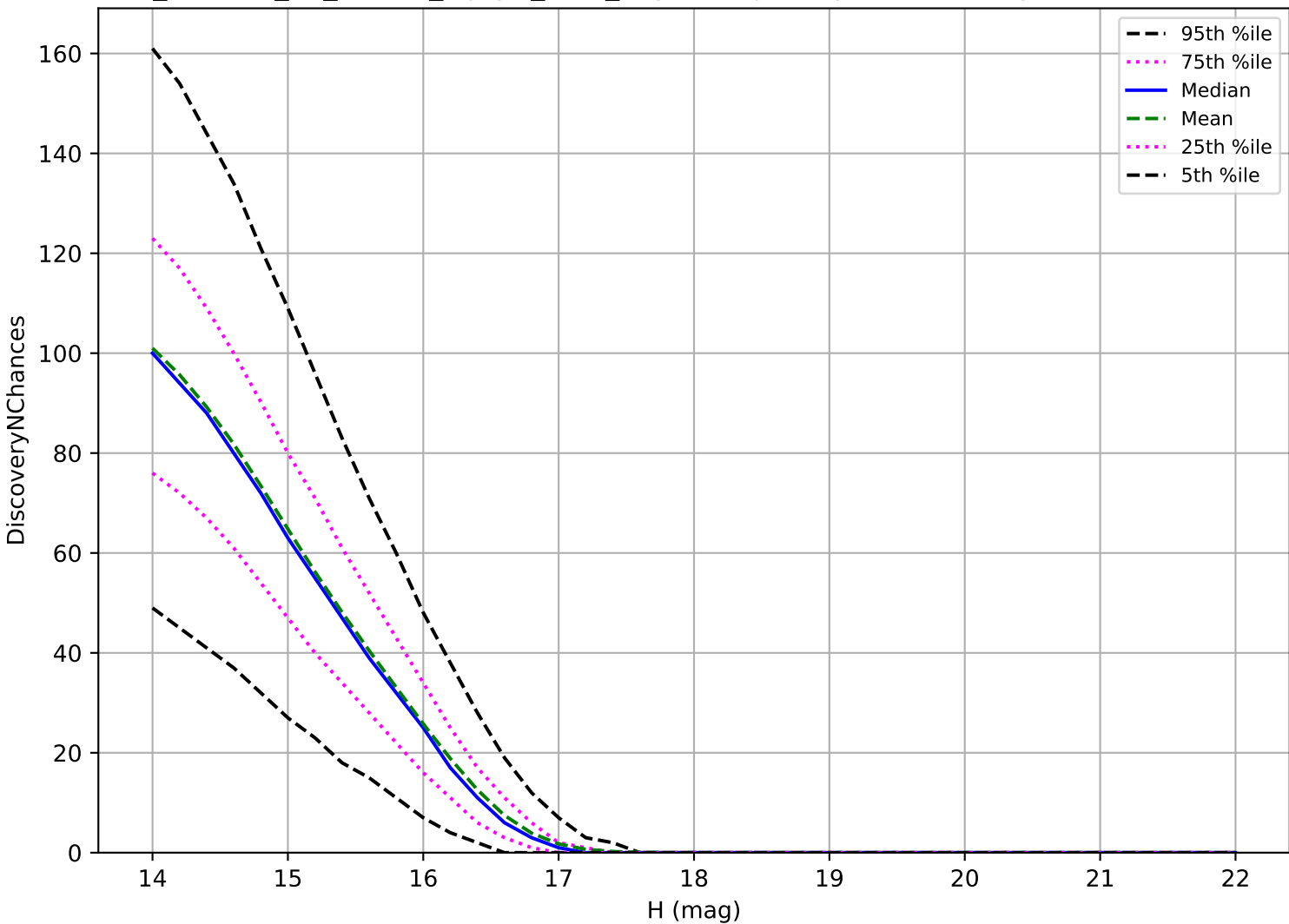
roll_uniform_eh_acc0.0_mjdp0_v3.4_10yrs: Trojan 3 pairs in 15 nights detection loss
