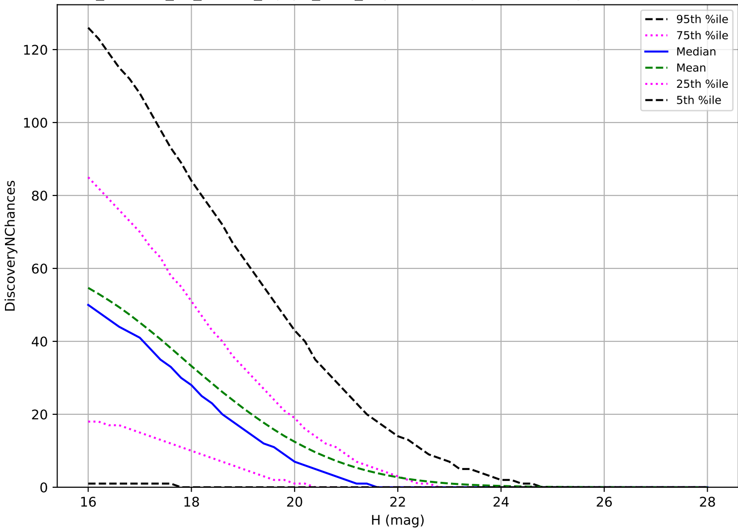
roll_uniform_eh_acc0.0_mjdp0_v3.4_10yrs: PHA 3 pairs in 15 nights detection loss
