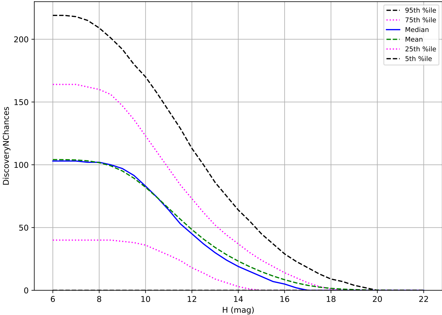
roll_uniform_eh_acc0.0_mjdp0_v3.4_10yrs: OCC_r5 3 pairs in 15 nights detection loss
