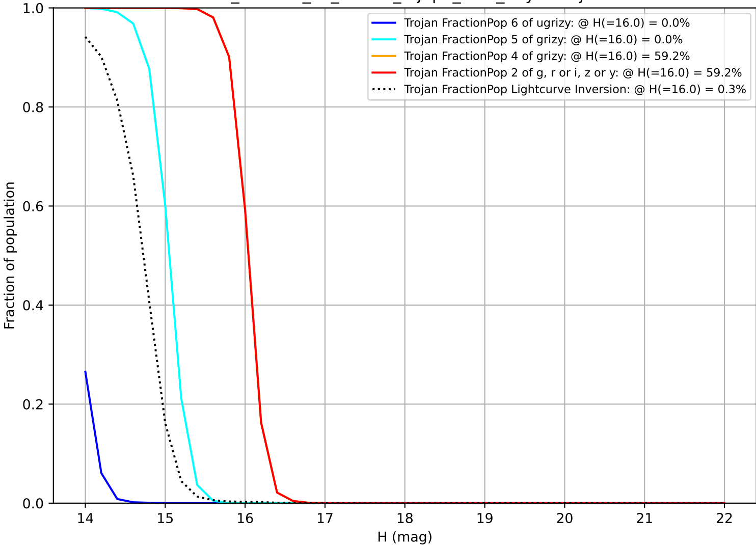
roll_uniform_eh_acc0.0_mjdp0_v3.4_10yrs Trojan
