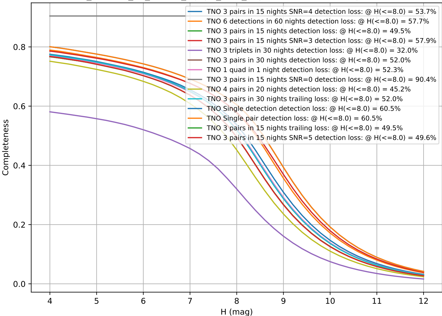
roll_uniform_eh_acc0.0_mjdp0_v3.4_10yrs: CumulativeCompleteness
