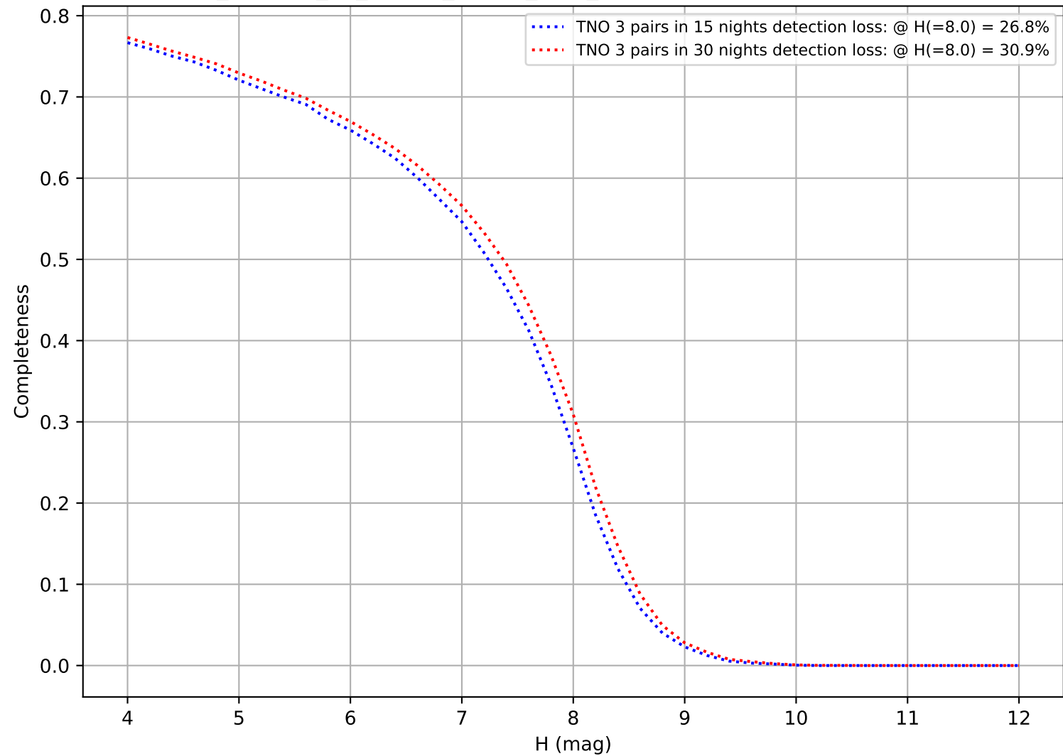
roll_uniform_eh_acc0.0_mjdp0_v3.4_10yrs: DifferentialCompleteness
