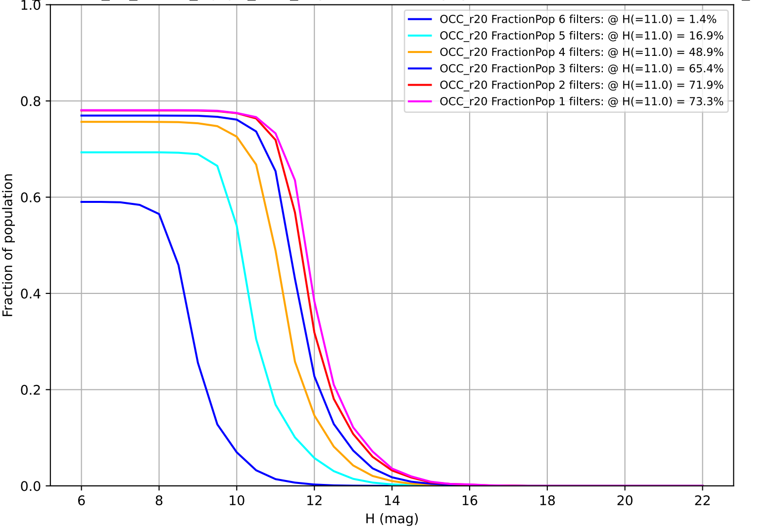
roll_uniform_eh_acc0.0_mjdp0_v3.4_10yrs: Fraction of population with colors in X filters OCC_r20
