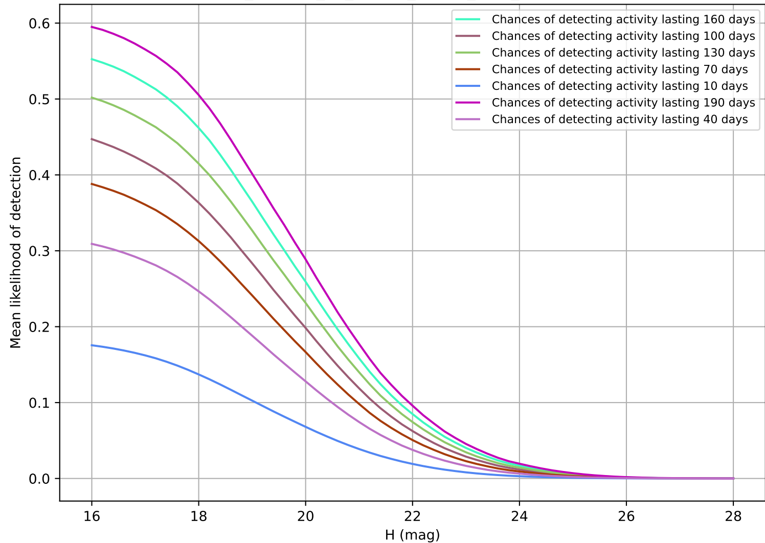
roll_uniform_eh_acc0.0_mjdp0_v3.4_10yrs NEO
