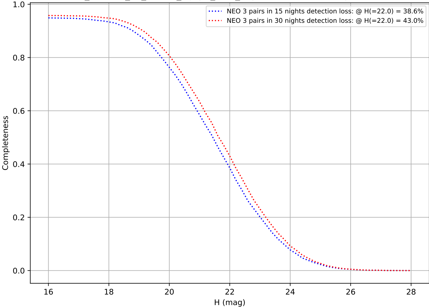
roll_uniform_eh_acc0.0_mjdp0_v3.4_10yrs: DifferentialCompleteness
