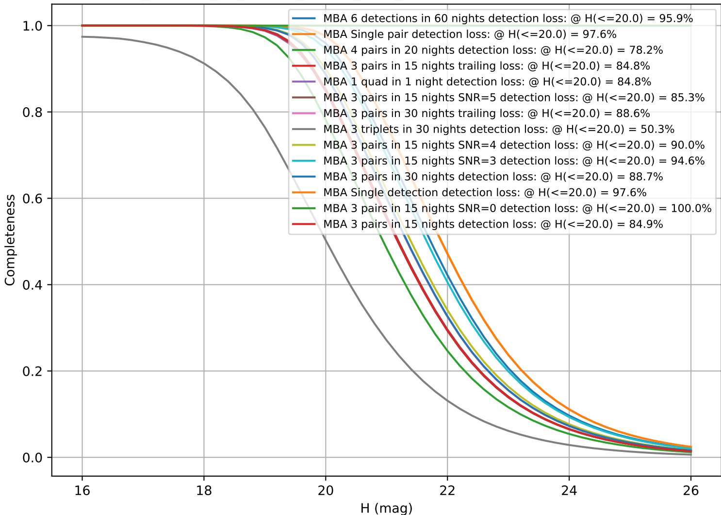
roll_uniform_eh_acc0.0_mjdp0_v3.4_10yrs: CumulativeCompleteness
