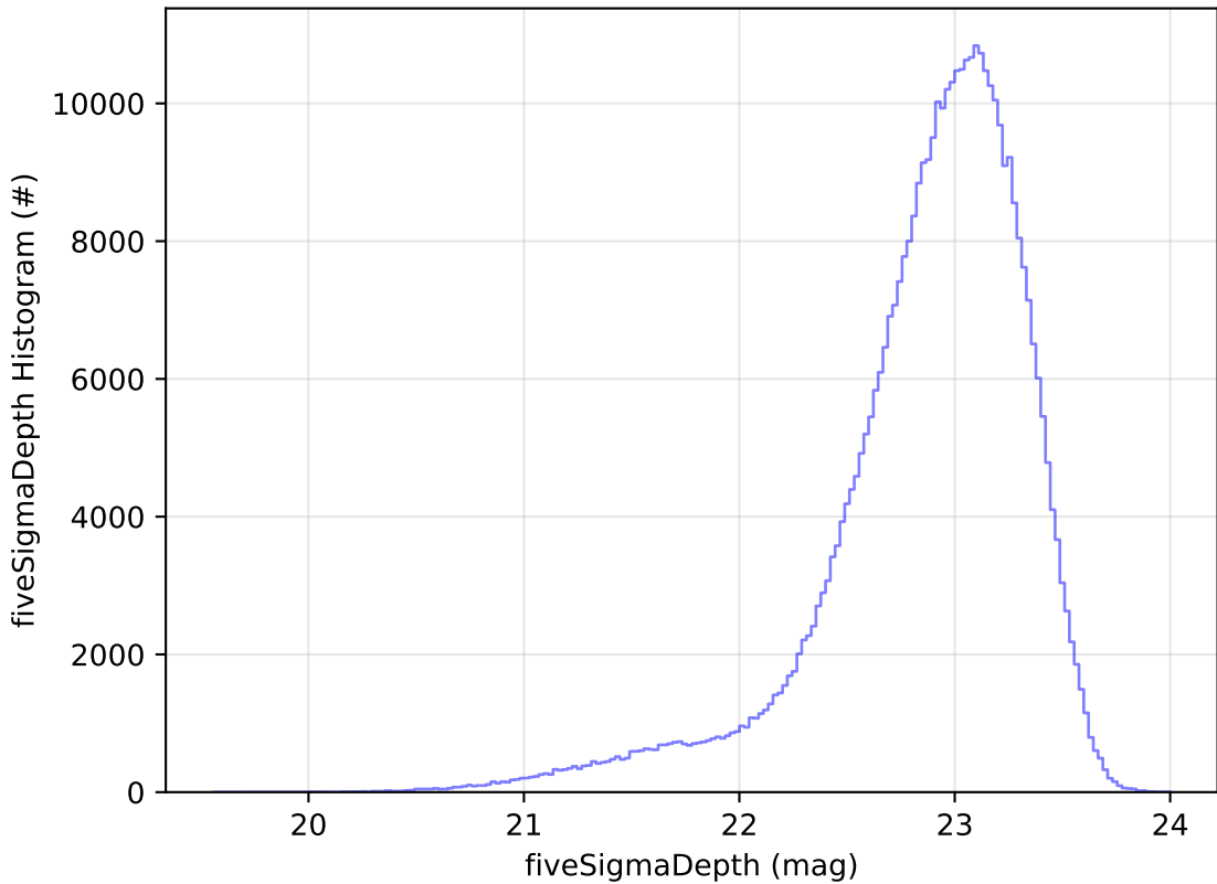
roll_uniform_eh_acc0.0_mjdp0_v3.4_10yrs z: fiveSigmaDepth Histogram
