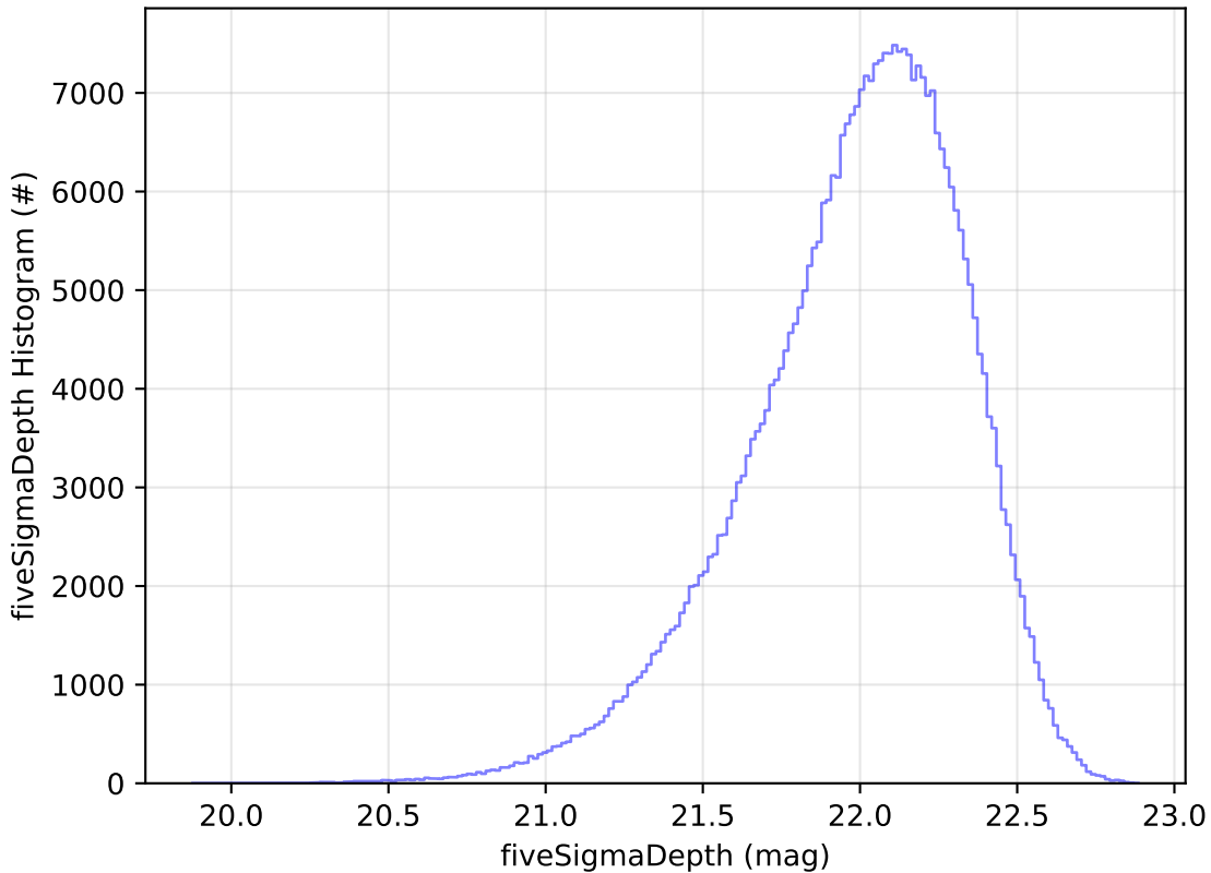
roll_uniform_eh_acc0.0_mjdp0_v3.4_10yrs y: fiveSigmaDepth Histogram
