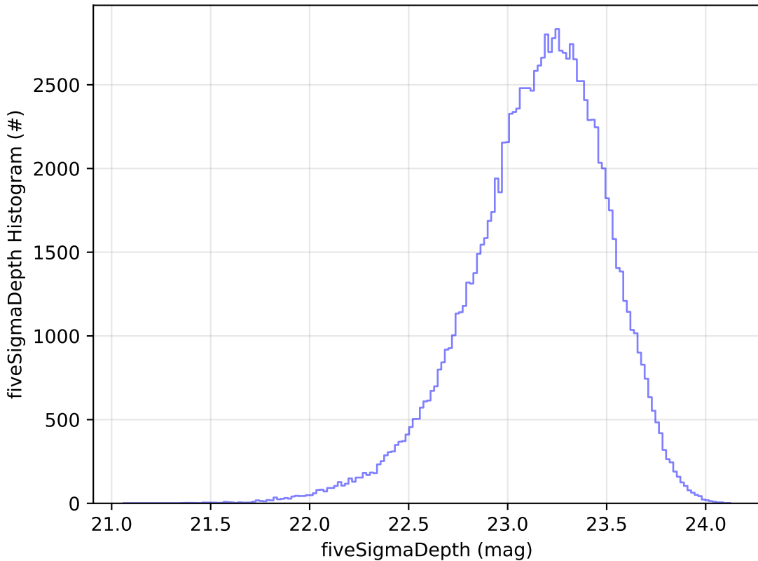
roll_uniform_eh_acc0.0_mjdp0_v3.4_10yrs u: fiveSigmaDepth Histogram
