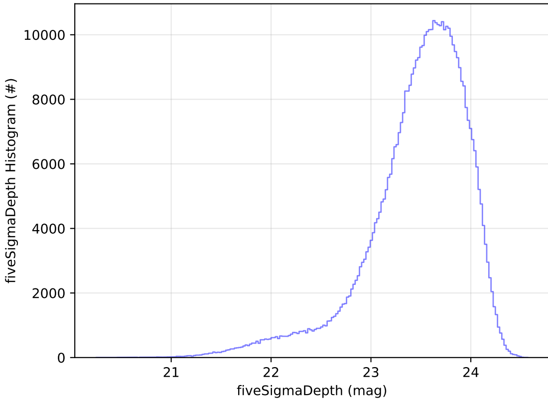
roll_uniform_eh_acc0.0_mjdp0_v3.4_10yrs i: fiveSigmaDepth Histogram
