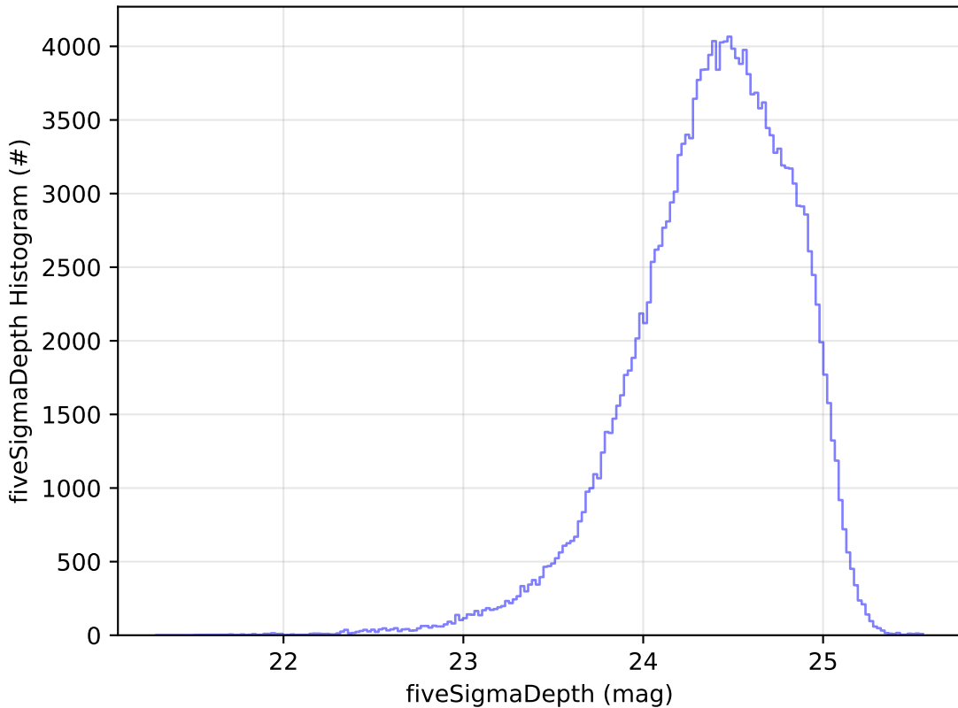
roll_uniform_eh_acc0.0_mjdp0_v3.4_10yrs g: fiveSigmaDepth Histogram
