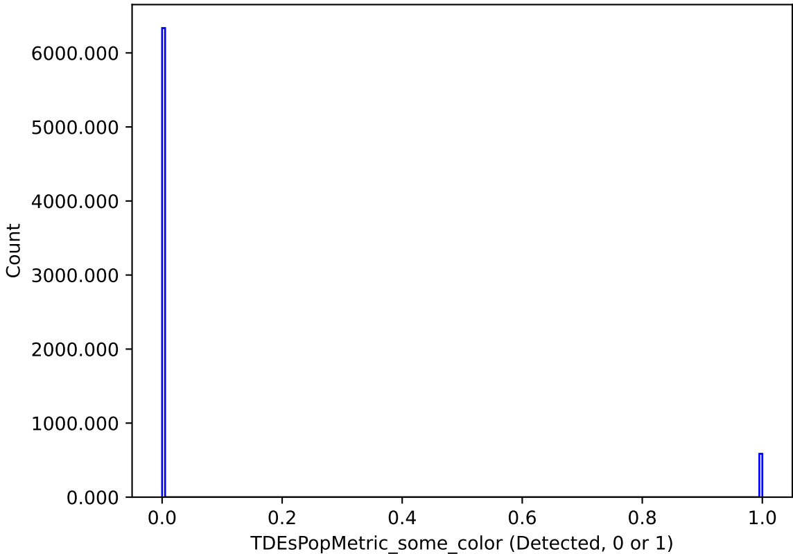
roll_uniform_eh_acc0.0_mjdp0_v3.4_10yrs : TDEsPopMetric_some_color
