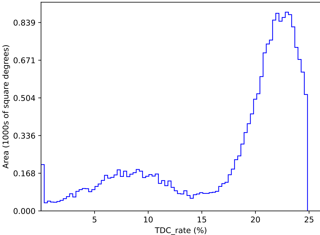
roll_uniform_eh_acc0.0_mjdp0_v3.4_10yrs : TDC_rate
