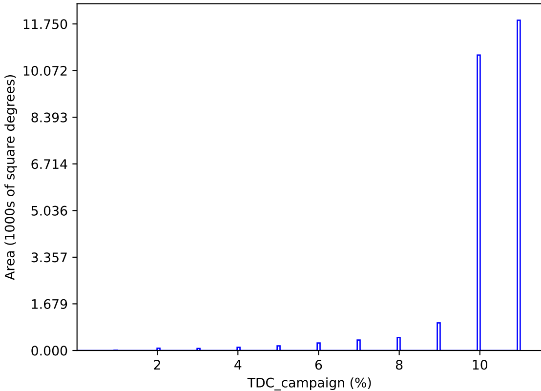
roll_uniform_eh_acc0.0_mjdp0_v3.4_10yrs : TDC_campaign
