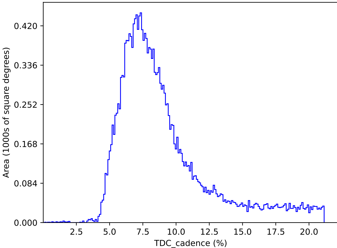
roll_uniform_eh_acc0.0_mjdp0_v3.4_10yrs : TDC_cadence
