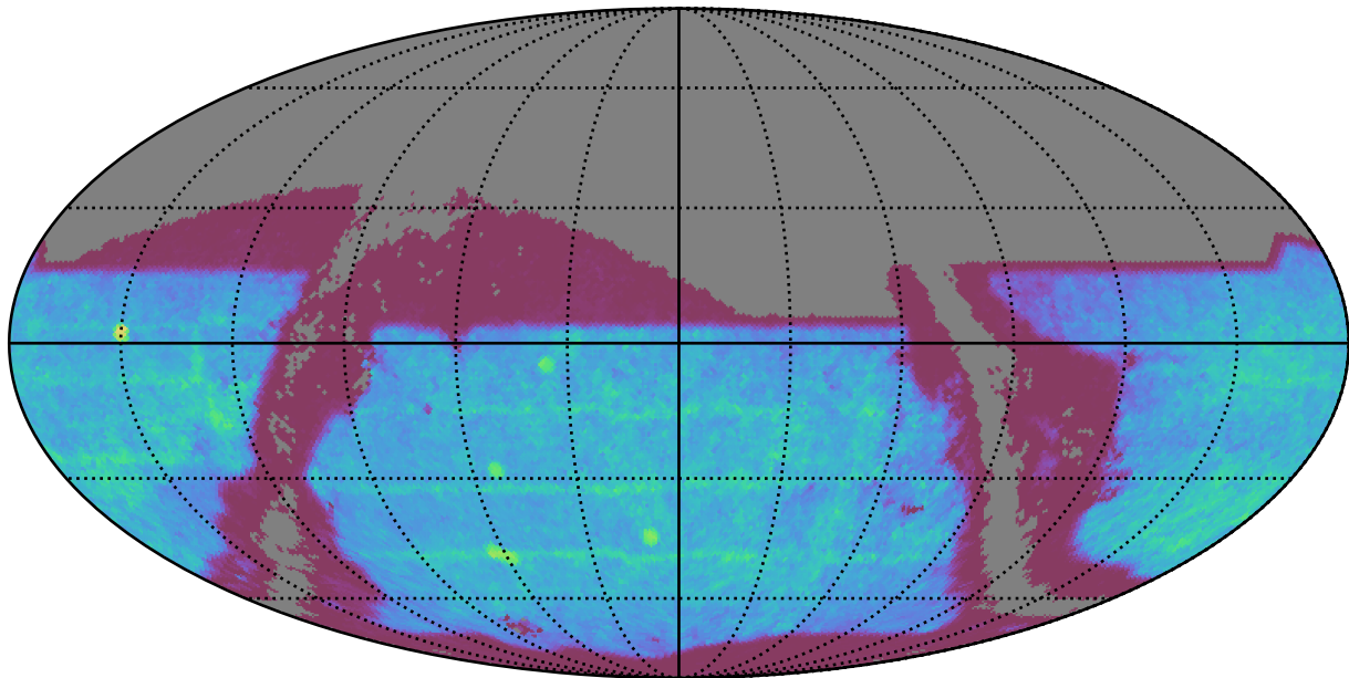
roll_uniform_eh_acc0.0_mjdp0_v3.4_10yrs : SNSLMetric
