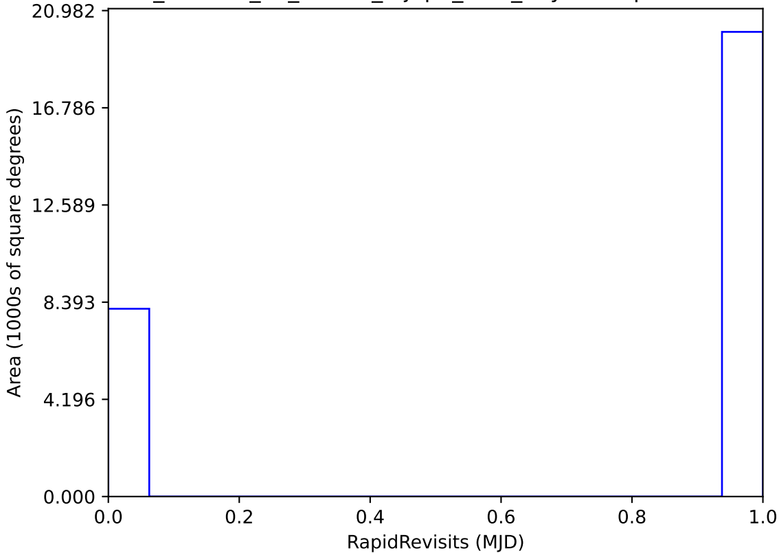
roll_uniform_eh_acc0.0_mjdp0_v3.4_10yrs : RapidRevisits
