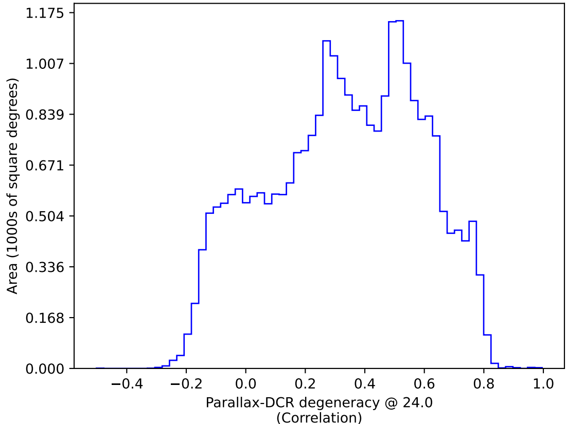
roll_uniform_eh_acc0.0_mjdp0_v3.4_10yrs : Parallax-DCR degeneracy @ 24.0
