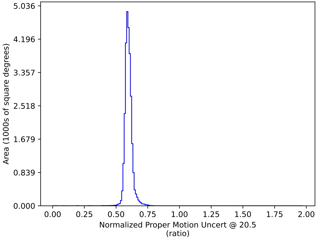
roll_uniform_eh_acc0.0_mjdp0_v3.4_10yrs : Normalized Proper Motion Uncert @ 20.5
