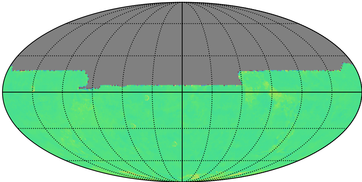
roll_uniform_eh_acc0.0_mjdp0_v3.4_10yrs y: Kuiper rotTelPos
