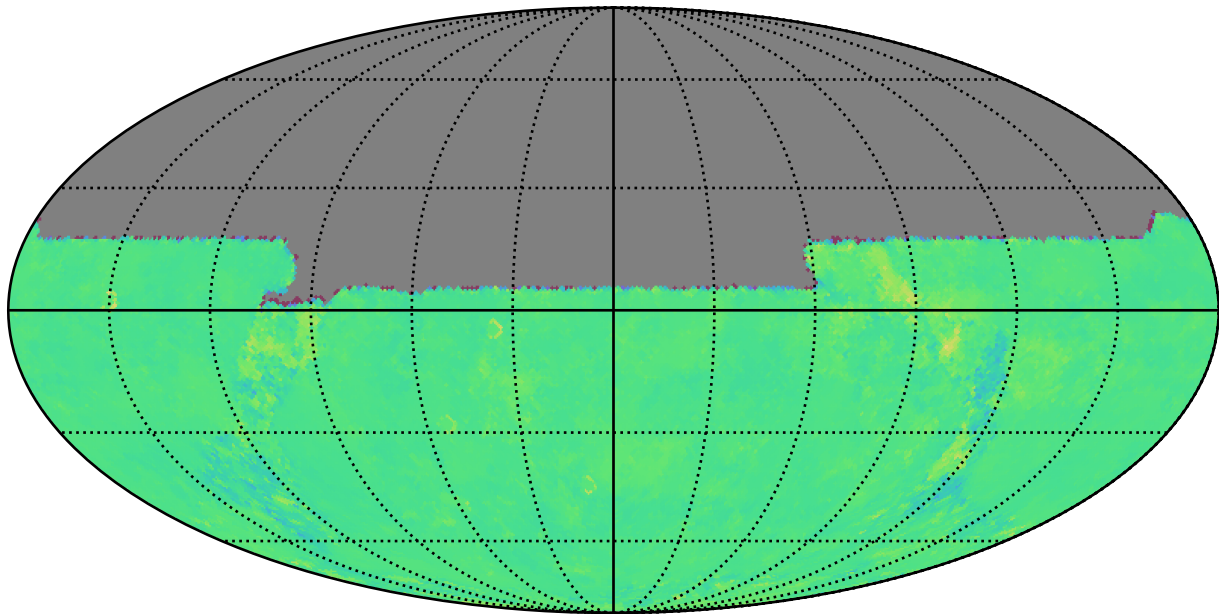
roll_uniform_eh_acc0.0_mjdp0_v3.4_10yrs u: Kuiper rotTelPos
