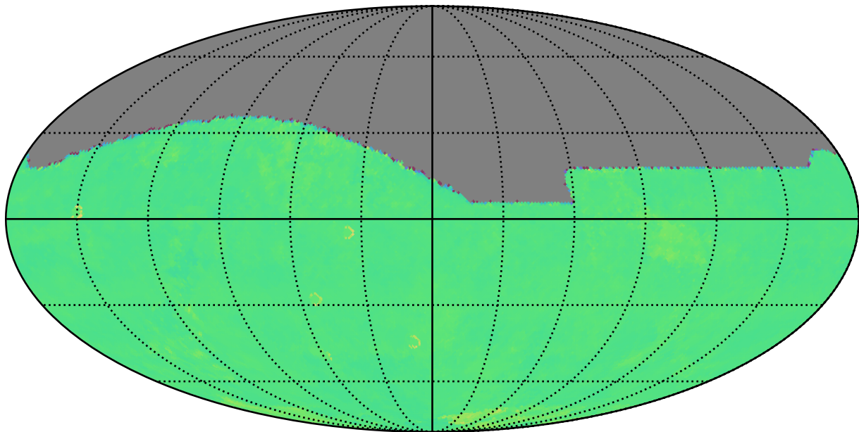
roll_uniform_eh_acc0.0_mjdp0_v3.4_10yrs r: Kuiper rotTelPos
