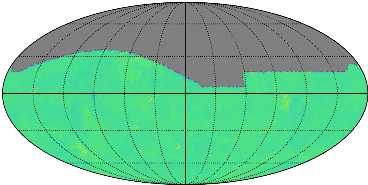
roll_uniform_eh_acc0.0_mjdp0_v3.4_10yrs g: Kuiper rotTelPos
