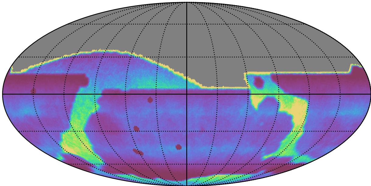
roll_uniform_eh_acc0.0_mjdp0_v3.4_10yrs : DCRprecision
