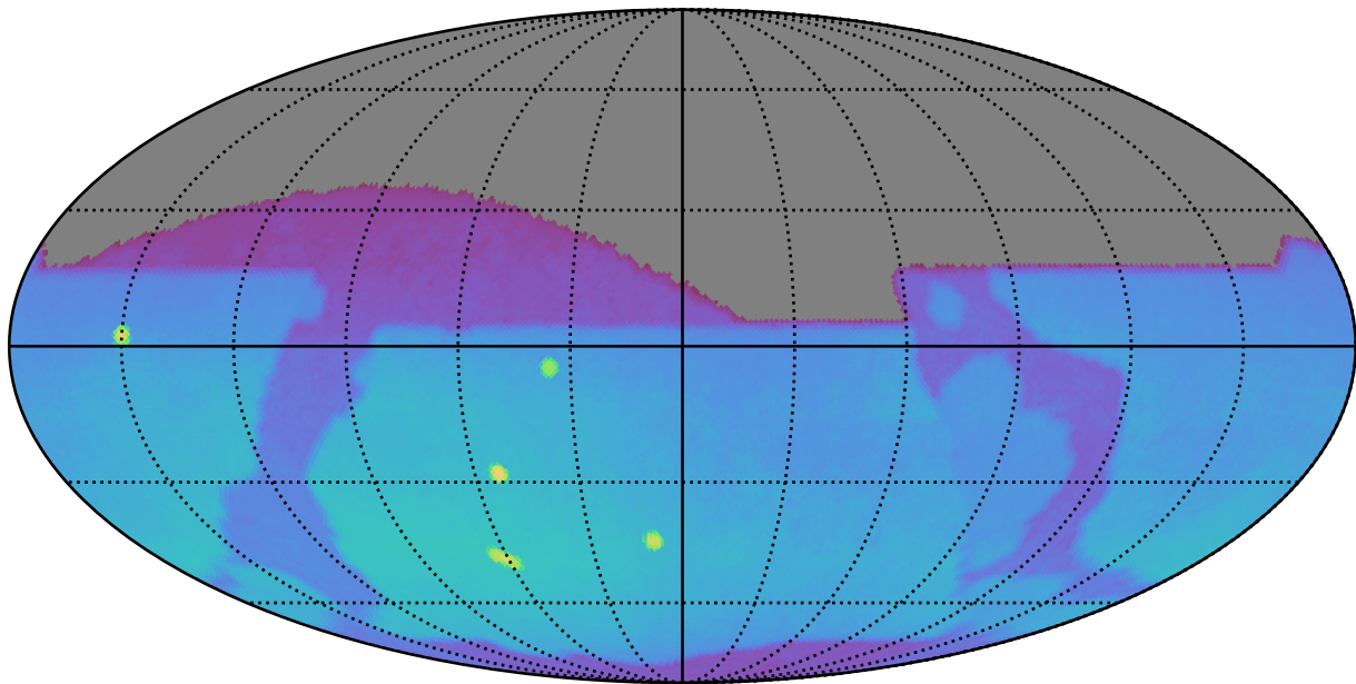
roll_uniform_eh_acc0.0_mjdp0_v3.4_10yrs : Brown Dwarf, L7
