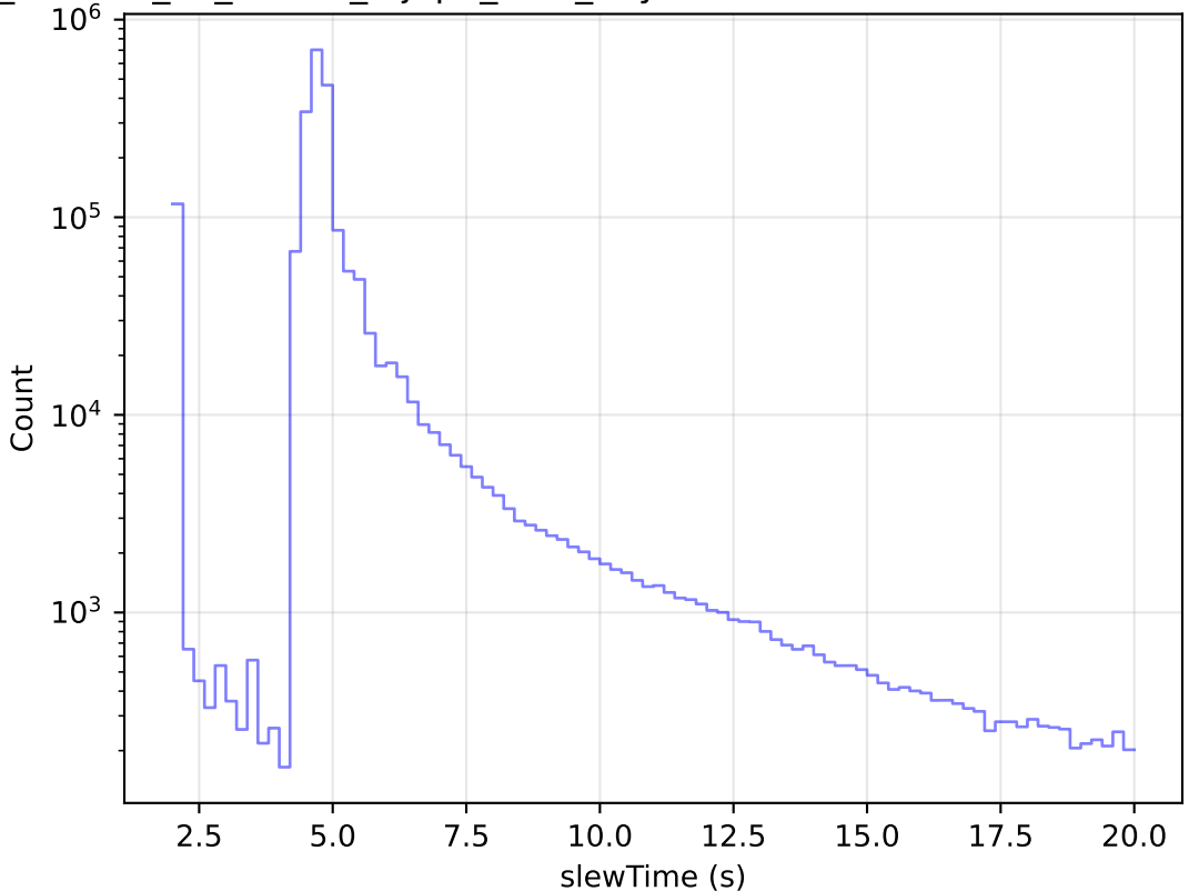
roll_uniform_eh_acc0.0_mjdp0_v3.4_10yrs All visits: Zoom Slew Time Histogram
