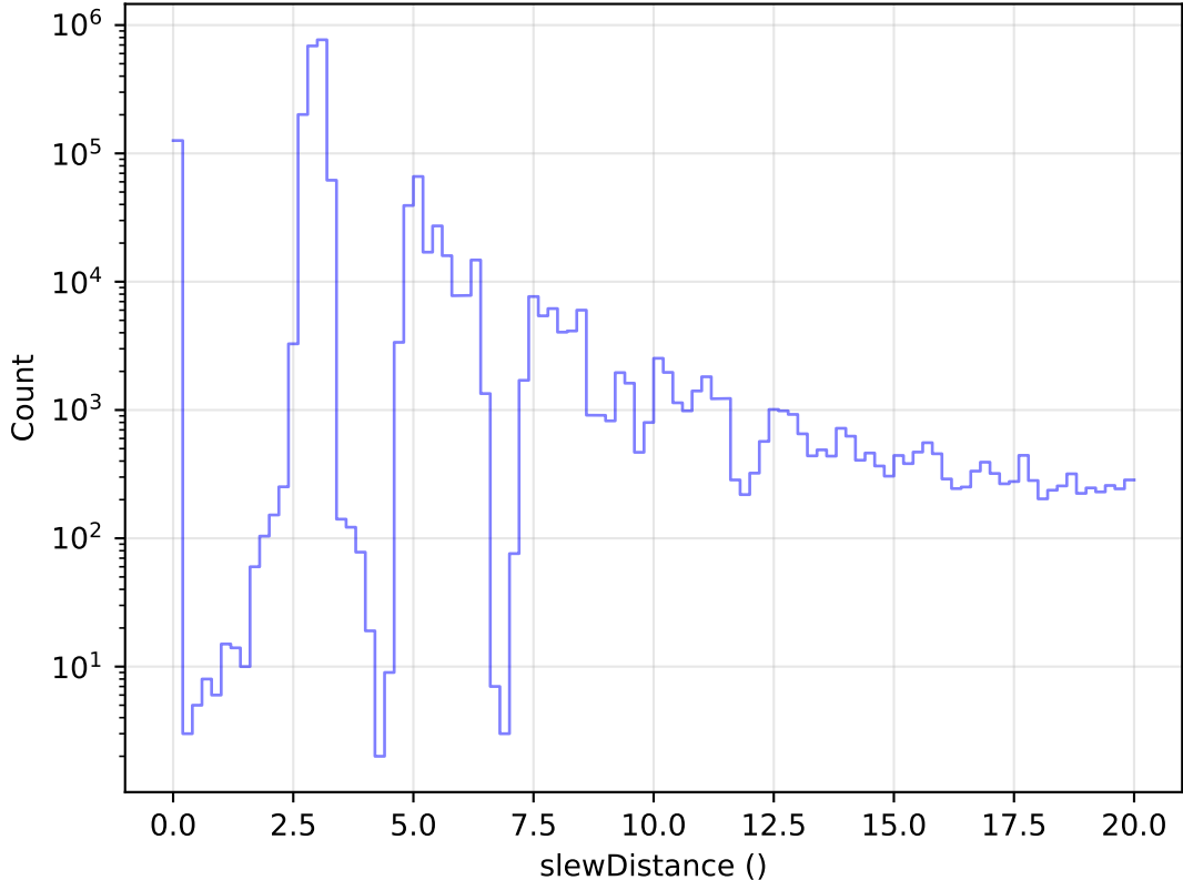
roll_uniform_eh_acc0.0_mjdp0_v3.4_10yrs All visits: Zoom Slew Distance Histogram
