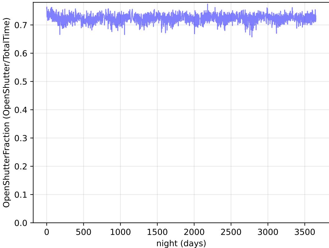
roll_uniform_eh_acc0.0_mjdp0_v3.4_10yrs : OpenShutterFraction
