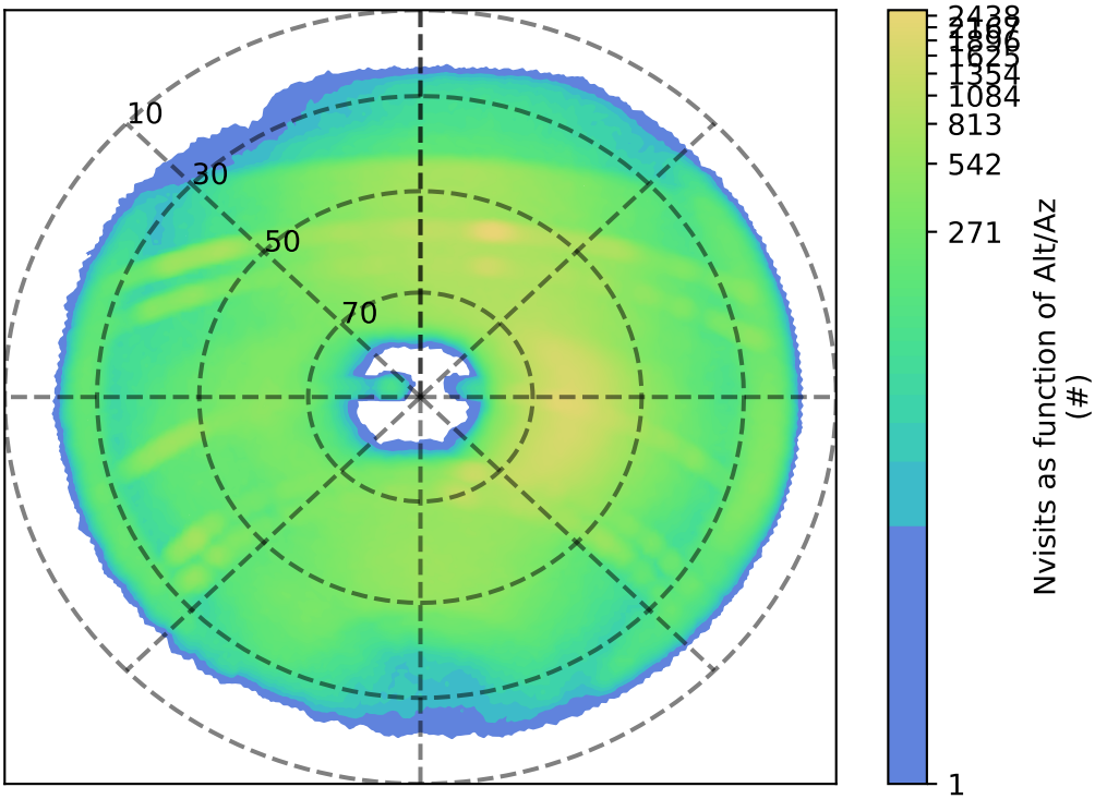
roll_uniform_eh_acc0.0_mjdp0_v3.4_10yrs z: Nvisits as function of Alt/Az
